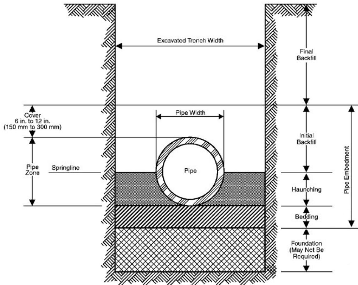
FIGURE 4: TRENCH CROSS-SECTION DIAGRAM
