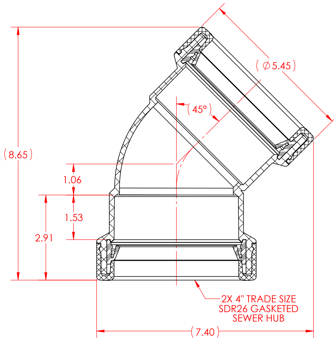
4" 1/8 BEND (45°) PVC SDR26 GASKETED SEWER 4"x 4" GxG
