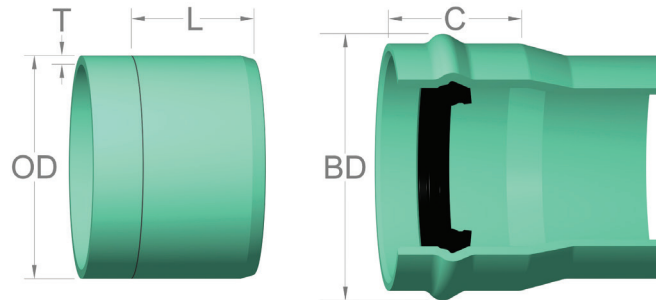
F679/IB PIPE DIMENSIONS &amp; PERFORMANCE
