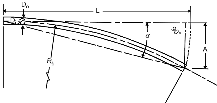
Figure 1: Longitudinal Bending Diagram (From PVC Pipe Association Handbook of PVC Pipe Design and Construction )
