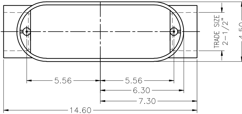
TOP VIEW W/O COVER
