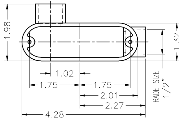
TOP VIEW W/O COVER
