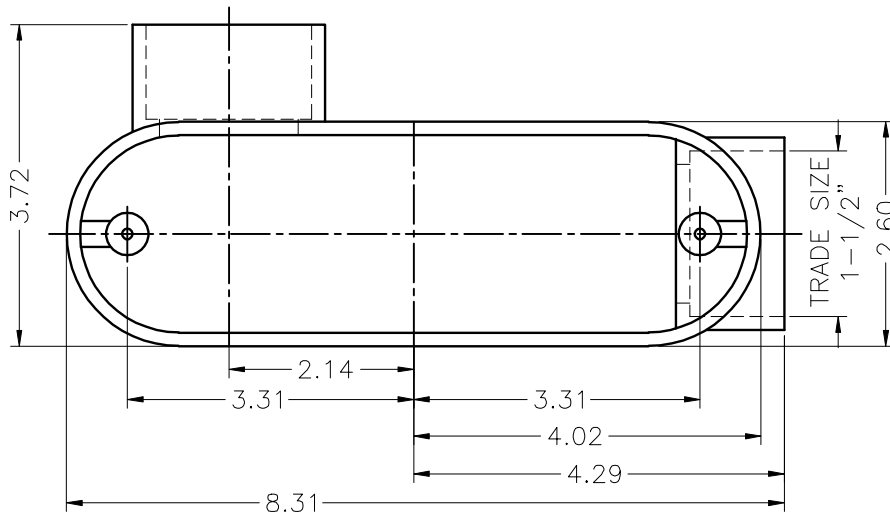
TOP VIEW W/O COVER
