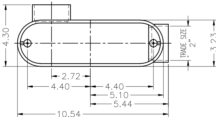
TOP VIEW W/O COVER
