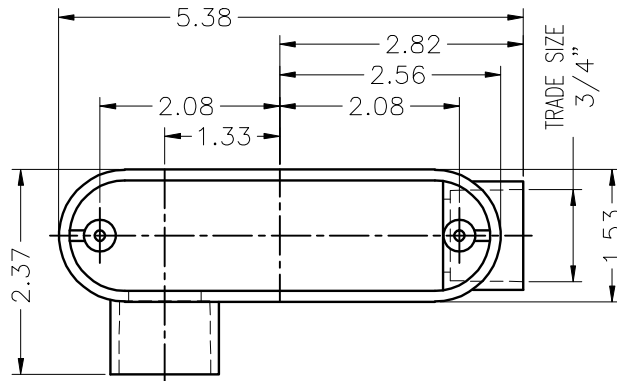
TOP VIEW W/O COVER
