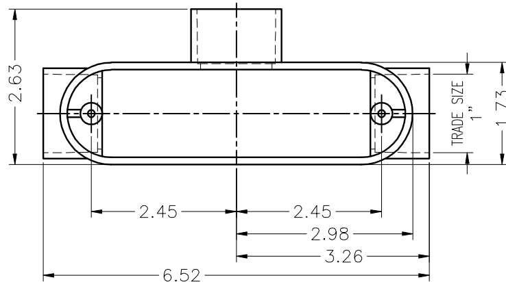
TOP VIEW W/O COVER
